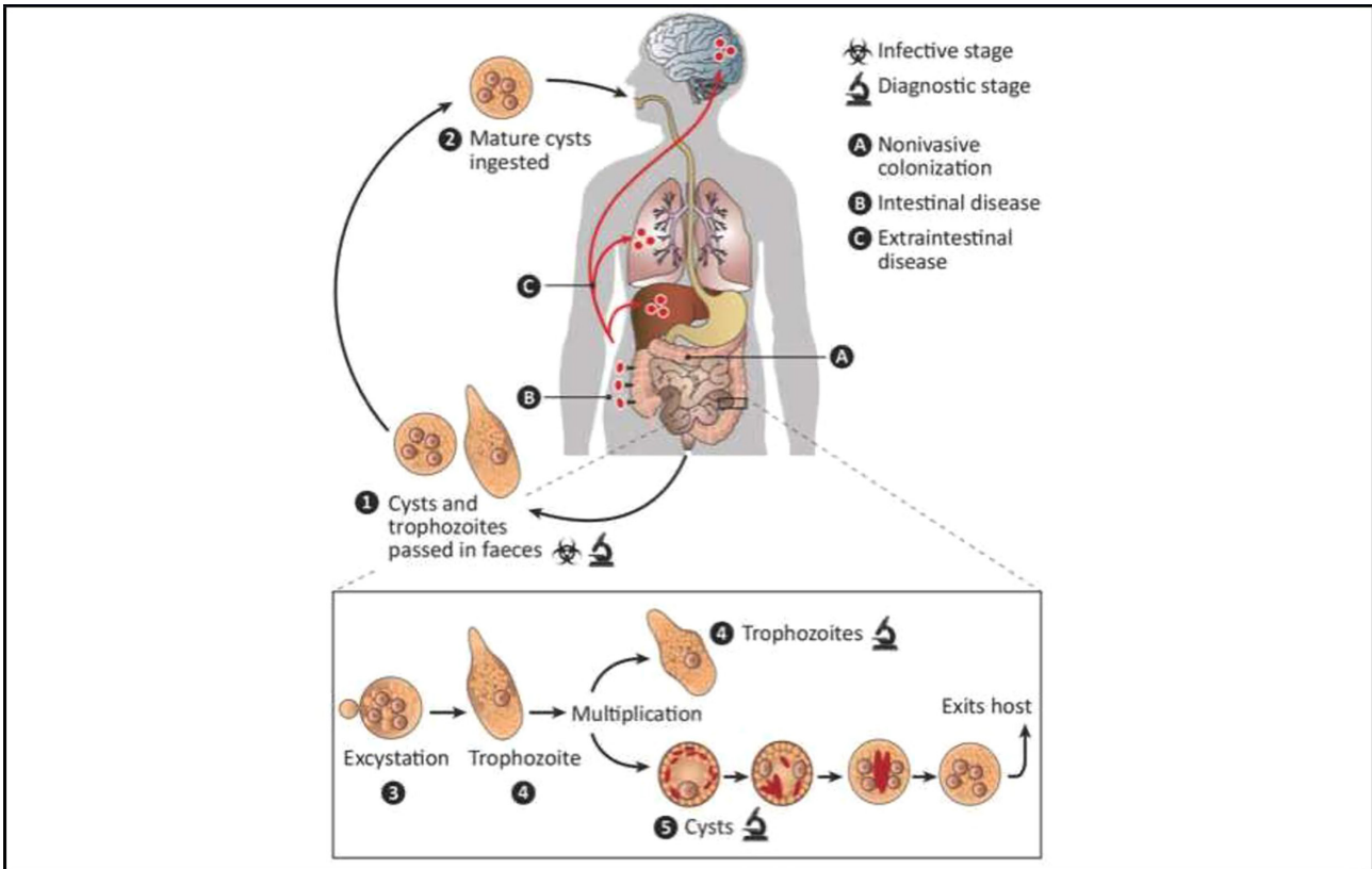
Figure 1 Entamoeba histolytica life cycle. Cysts and trophozoites are passed in faeces (1). Cysts are typically found in formed stool, whereas trophozoites are typically found in diarrhoeal stool. Infection with Entamoeba histolytica (and E. dispar ) occurs via ingestion of mature cysts (2) from faecally contaminated food, water, or hands. Exposure to infectious cysts and trophozoites in faecal matter during sexual contact may also occur. Excystation (3) occurs in the small intestine and trophozoites (4) are released, which migrate to the large intestine. Trophozoites may remain confined to the intestinal lumen (A): non-invasive infection) with individuals continuing to pass cysts in their stool (asymptomatic carriers). Trophozoites can invade the intestinal mucosa (B): intestinal disease), or blood vessels, reaching extraintestinal sites such as the liver, brain, and lungs (C): extraintestinal disease). Trophozoites multiply by binary fission and produce cysts (5), and both stages are passed in the faeces (1). Cysts can survive days to weeks in the external environment and remain infectious in the environment due to the protection conferred by their walls. Trophozoites passed in the stool are rapidly destroyed once outside the body, and if ingested would not survive exposure to the gastric environment. Adapted from source: CDC (Centers for Disease Control and Prevention, Atlanta, Georgia, USA): https://www.cdc.gov/dpdx/amebiasis/
